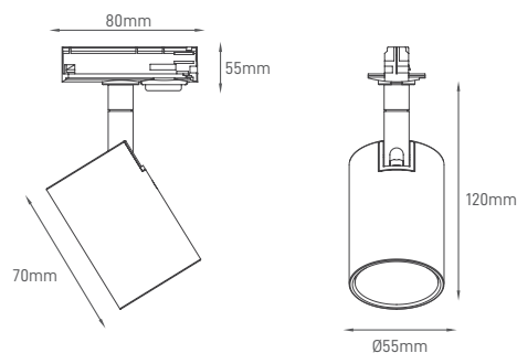
TECHNICAL DRAWING
