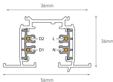
TECHNICAL DRAWING - RECESSED
