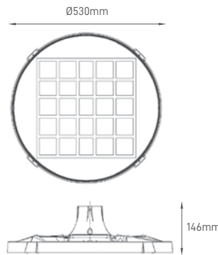
TECHNICAL DRAWING
