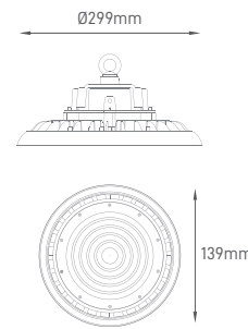
TECHNICAL DRAWING
