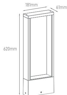
TECHNICAL DRAWING
