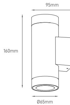
TECHNICAL DRAWING
