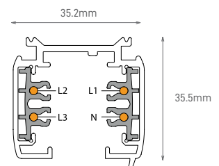
TECHNICAL DRAWING - SURFACE
