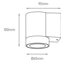
TECHNICAL DRAWING
