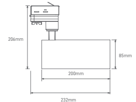
TECHNICAL DRAWING - CCT
